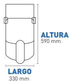
VISTA FRONTAL
